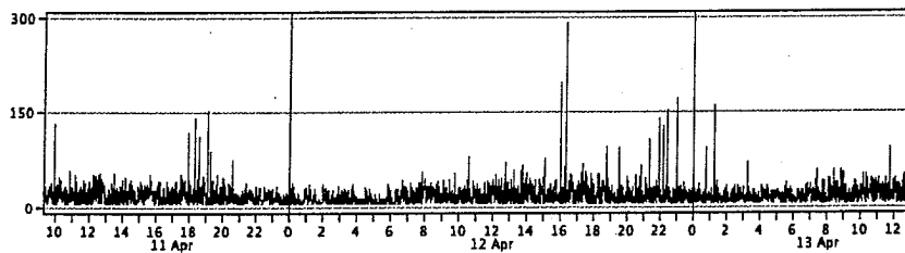
Figure 40: NMS graph round-trip ping times reporting health of wireless link.
